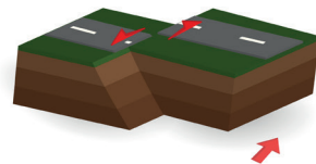
STRIKE-SLIP FAULT
